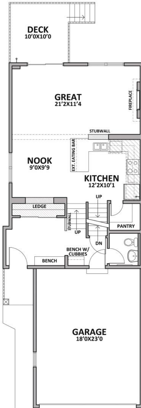
MAIN FLOOR 755 SQ.FT.
