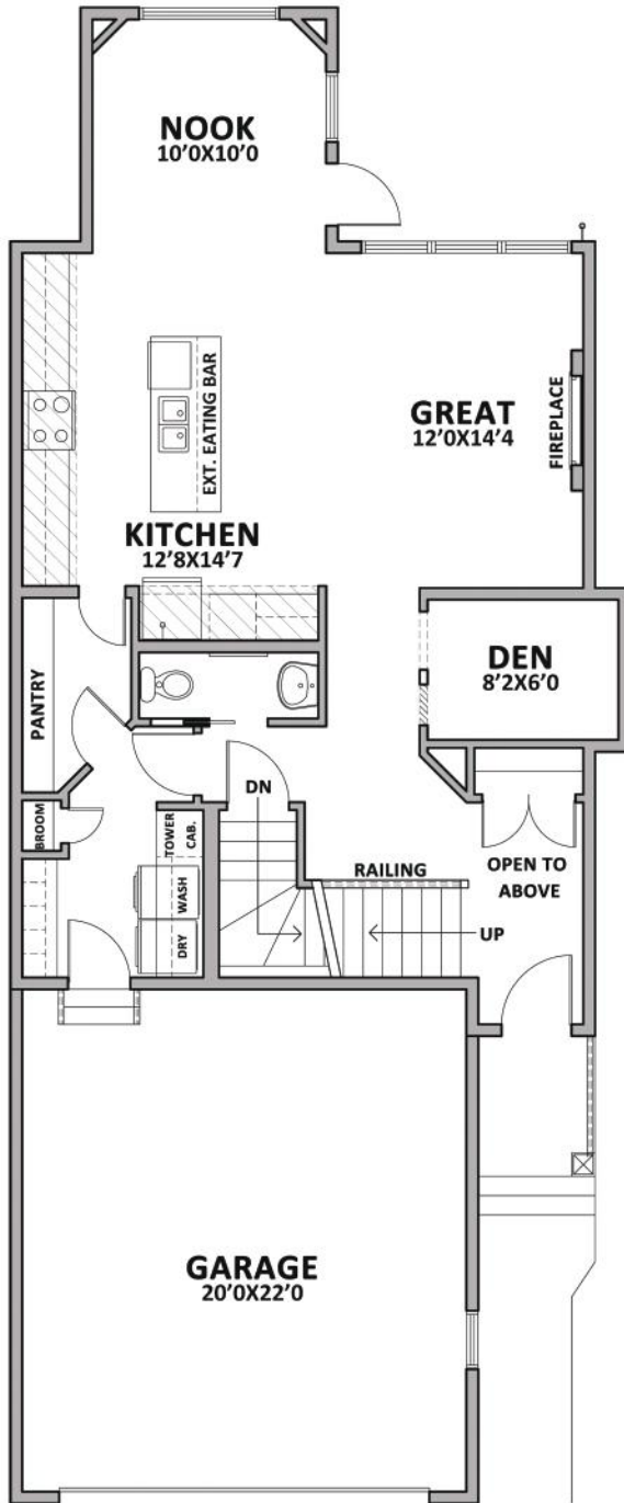
MAIN FLOOR 933 SQ.FT.
