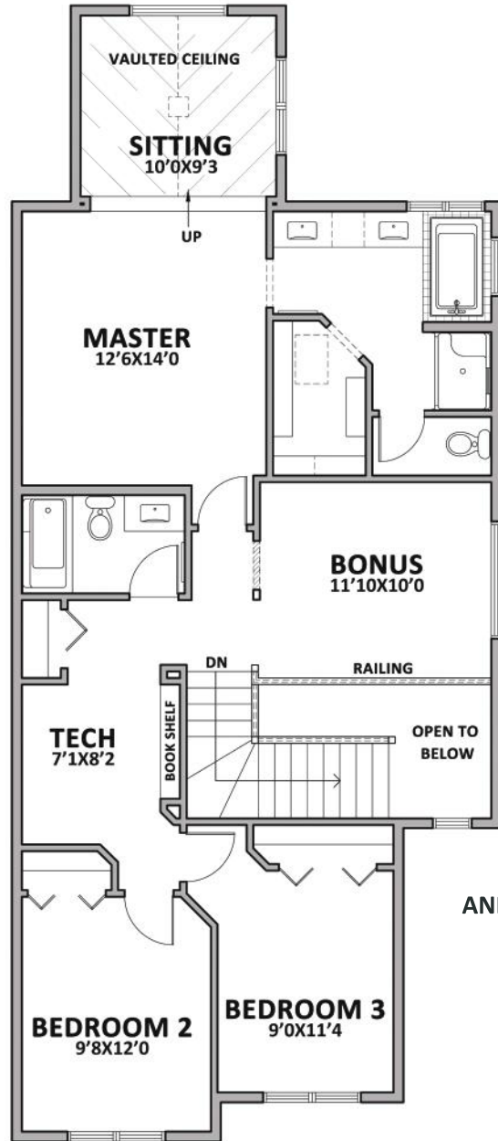
UPPER FLOOR 1103 SQ. FT.
